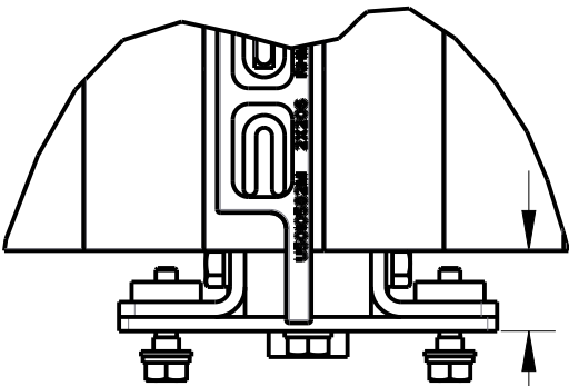
DETAIL D ECHELLE 3/8
